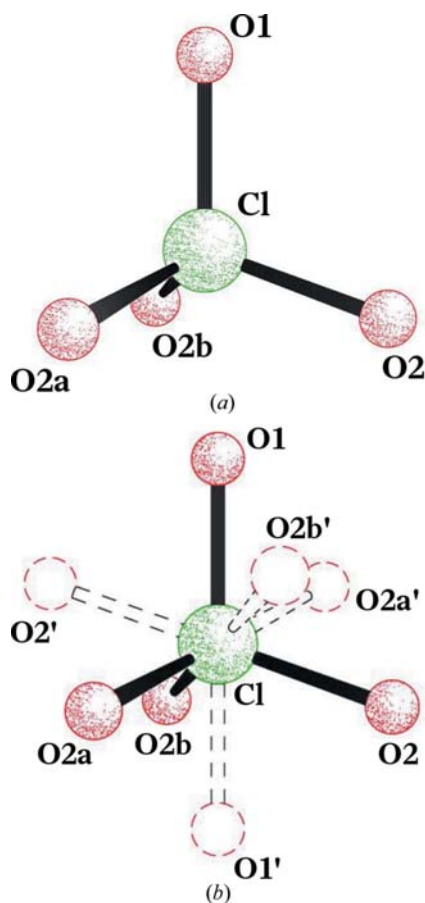
Figure 4 (a) A (rare) undistorted perchlorate anion on a threefold axis. Atoms O1 and Cl lie on this axis, O2a and O2b are symmetry equivalents of O2. (b) A (more common) disordered perchlorate anion. It still lies on a threefold axis, but there is a second orientation with atoms O1', O2a', O2b' etc.
